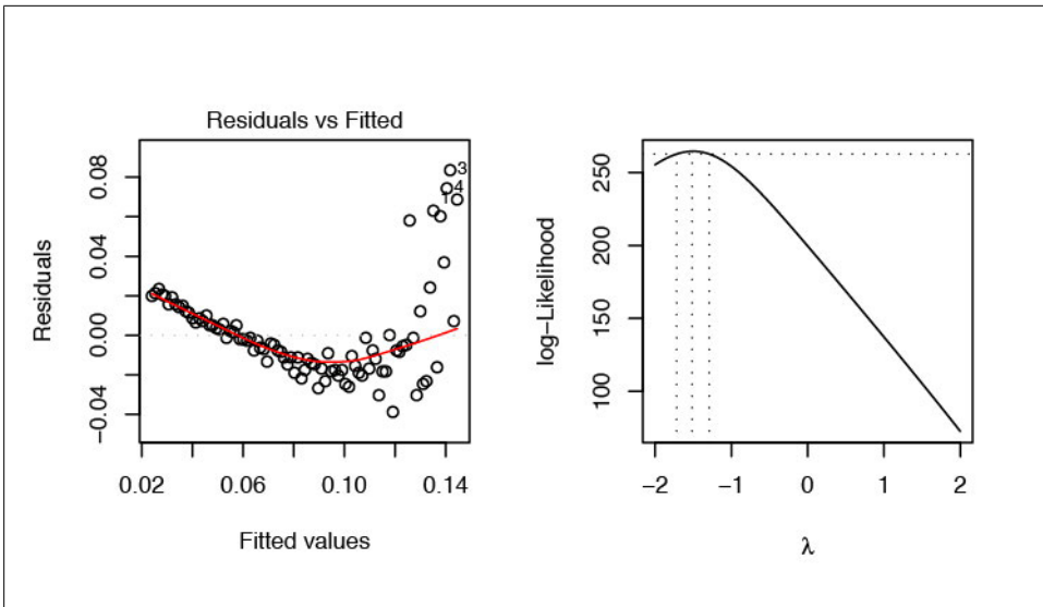
Figure 11-2. Box-Cox plots
