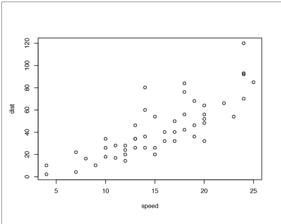
Figure 10-1. Scatter plot
