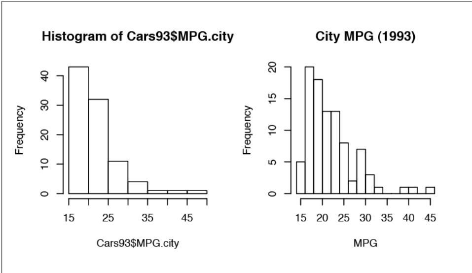
Figure 10-17. Histograms
