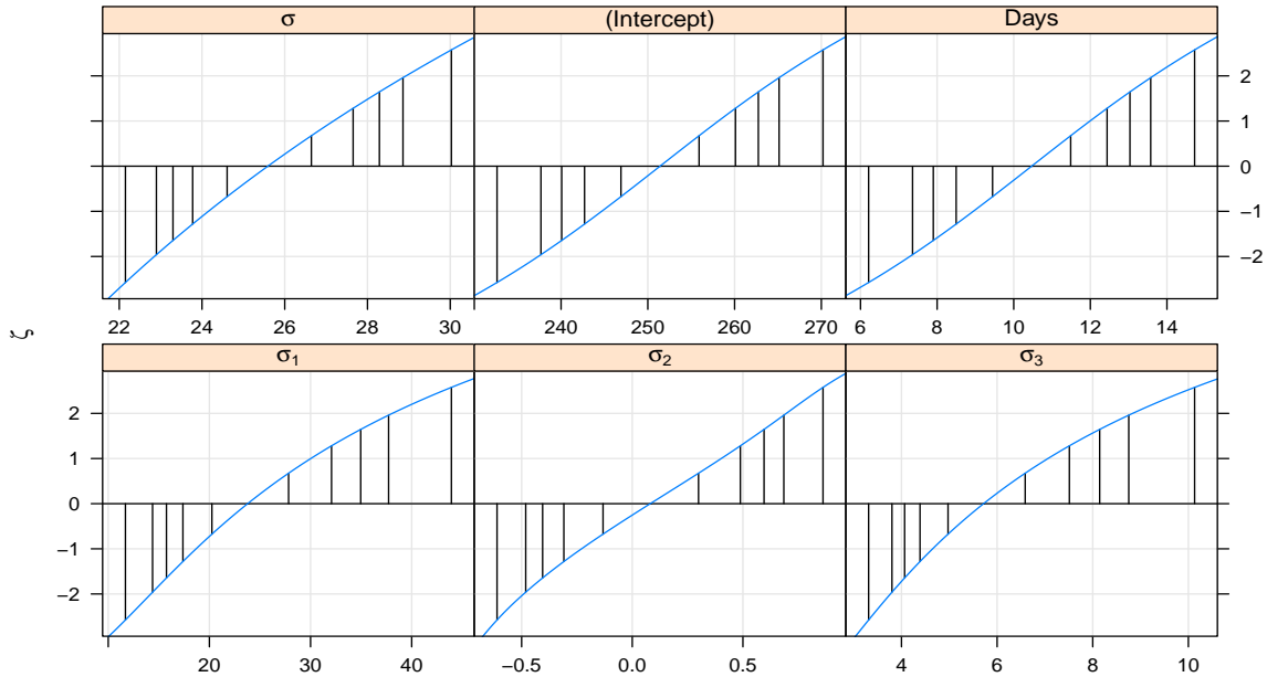
Figure 2: Profile zeta plot: xyplot(profile.obj)
